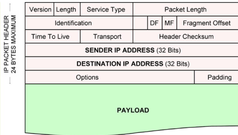
IPV4 data packet header.
